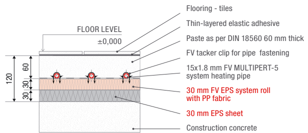
Figure 17: Recommended floor structure above cellar or occasionally heated rooms built terrain as per DIN EN 1264 norm recommendation, insulation heat resistance R = 1,25 m 2 K/W
